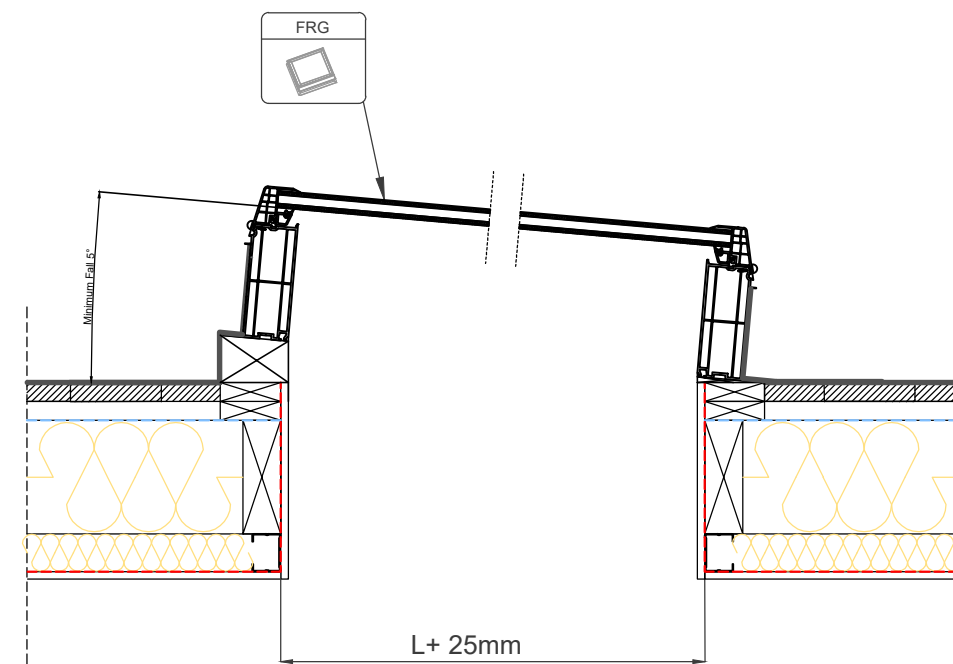
Section B-B' 1:10
