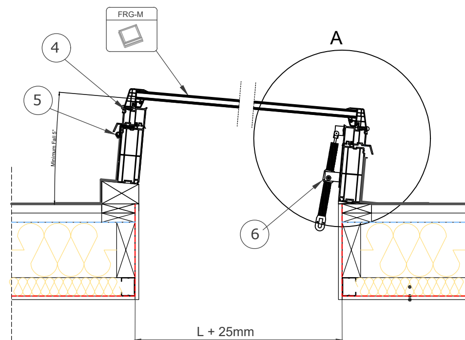
Section B-B' 1:10
