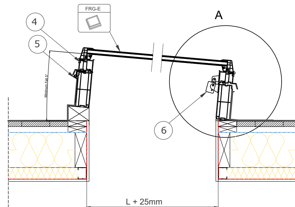
Section B-B' 1:10
