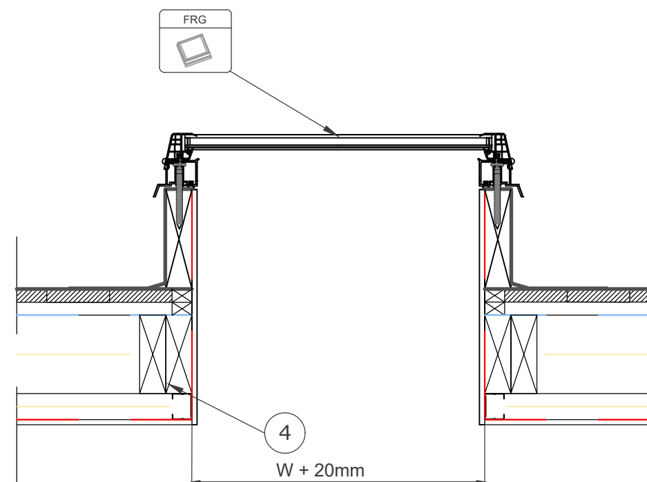
Section B-B' 1:10
