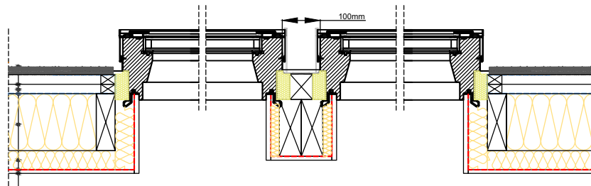
Section B-B' 1:10
