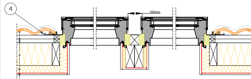
Section B-B' 1:10
