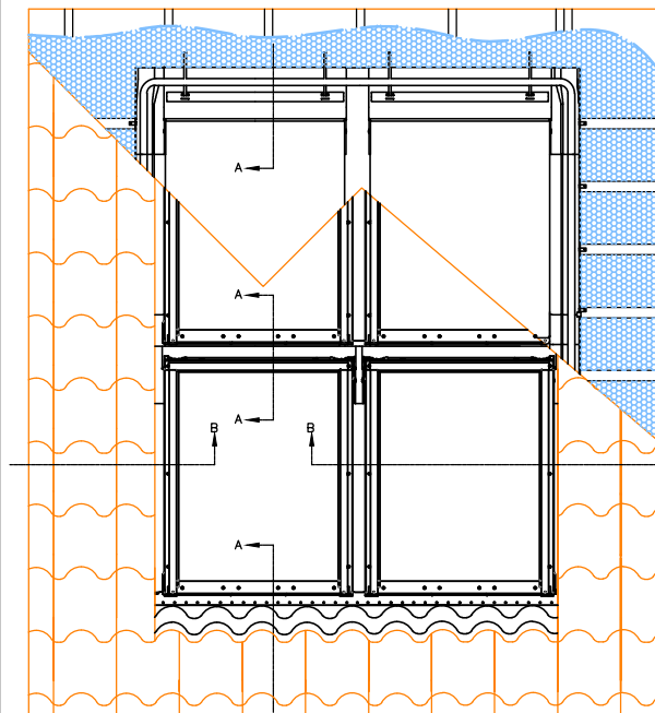
INDICATIVE SECTIONAL VIEW
