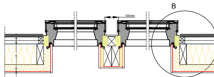
Section B-B' 1:10
