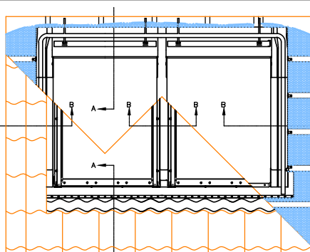
INDICATIVE SECTIONAL VIEW
