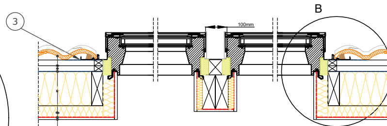
Section B-B' 1:10
