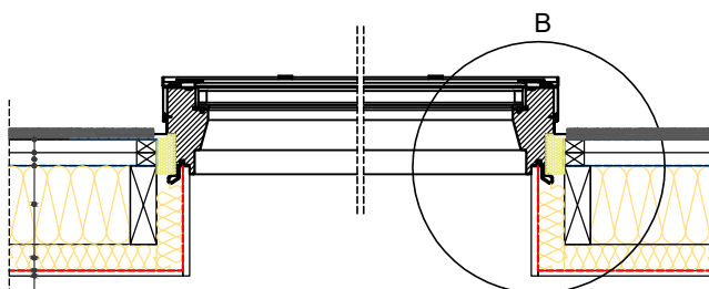
Section B-B' 1:10
