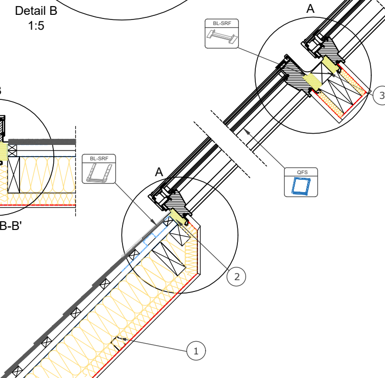
Detail A 1:5
