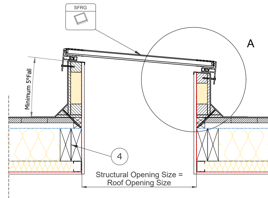
Section B-B' 1:10
