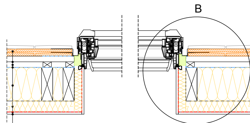
Section B-B' 1:10
