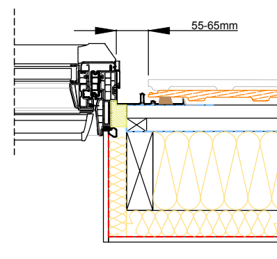
Section B-B' 1:10
