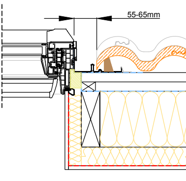
Section B-B' 1:10
