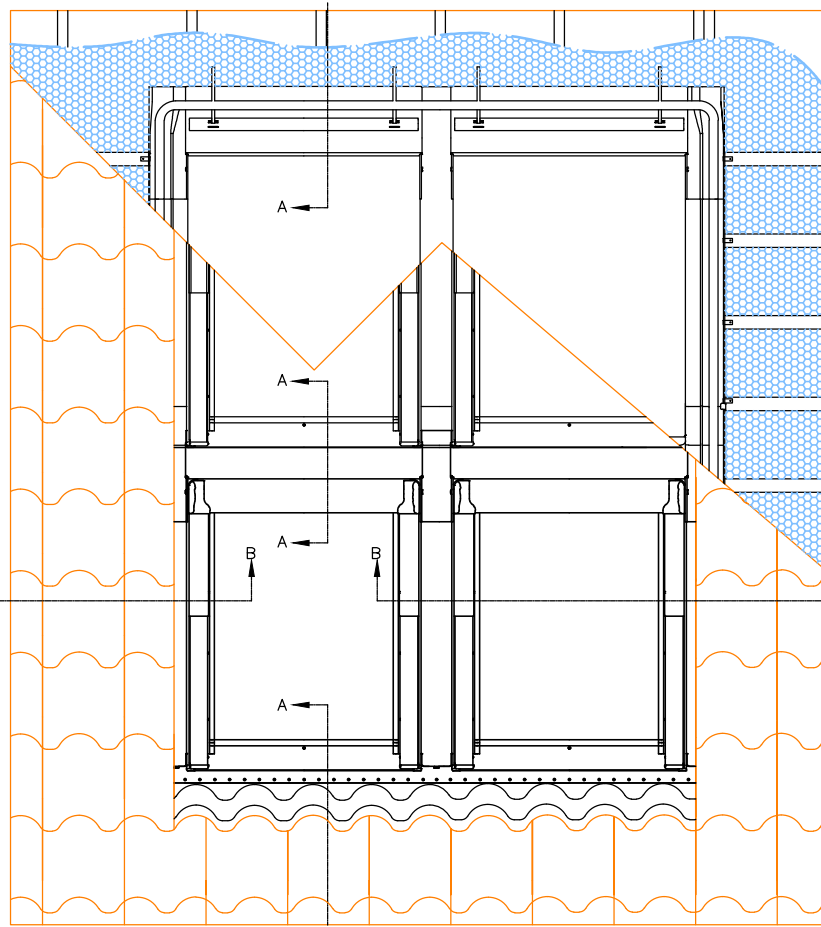
INDICATIVE SECTIONAL VIEW
