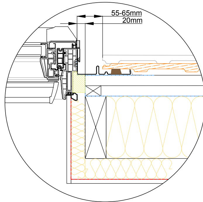
Detail B 1:5
