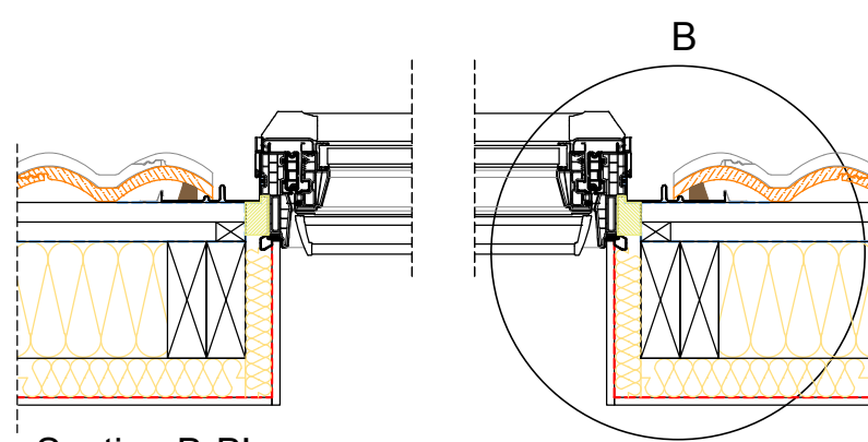
Section B-B' 1:10
