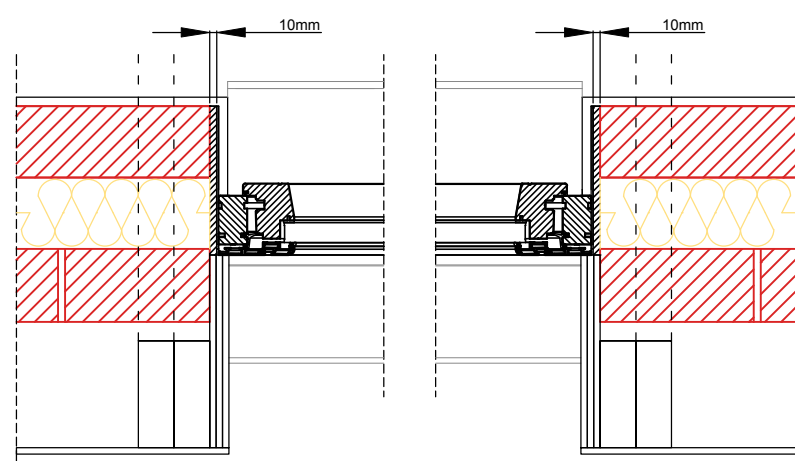
Section C-C' 1:10
