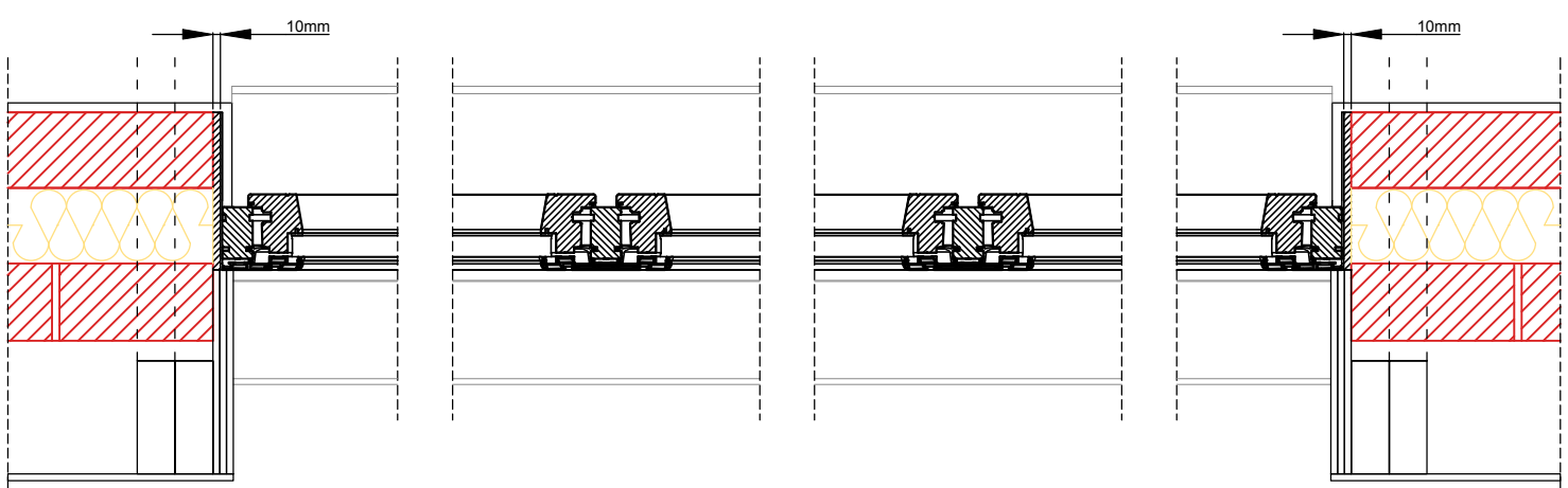
Section C-C' 1:10
