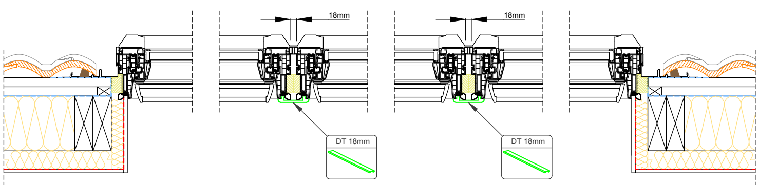
Section B-B' 1:10
