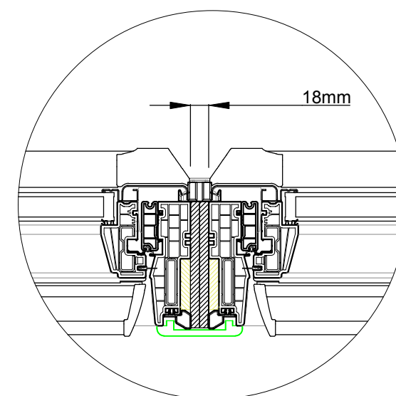
Detail A 1:5
