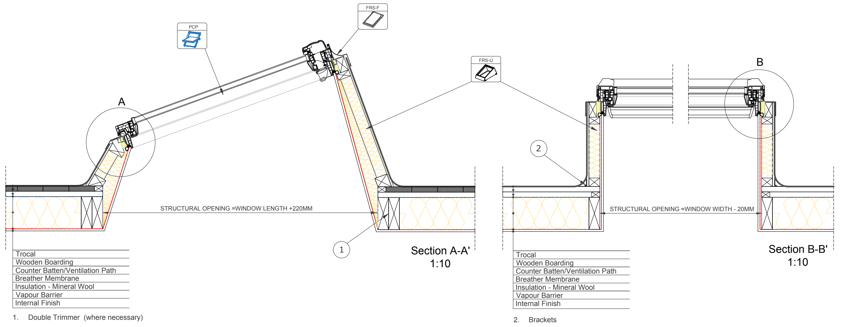
INDICATIVE SECTIONAL VIEW
