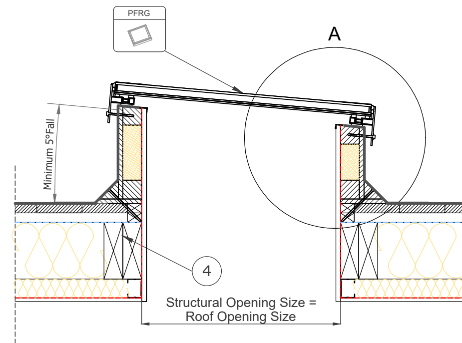
Section B-B' 1:10
