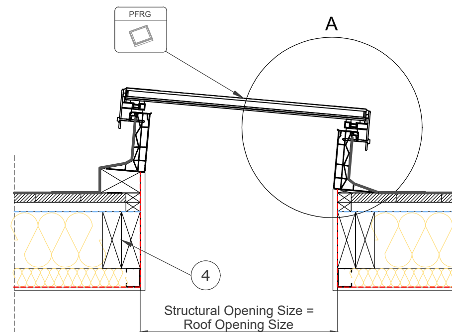
Section B-B' 1:10
