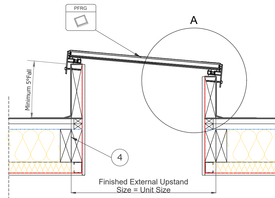
Section B-B' 1:10
