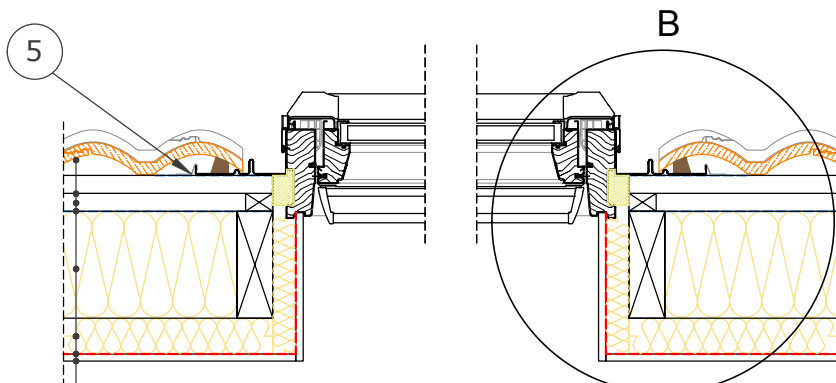
Section B-B' 1:10
