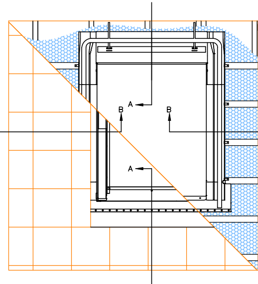
INDICATIVE SECTIONAL VIEW
