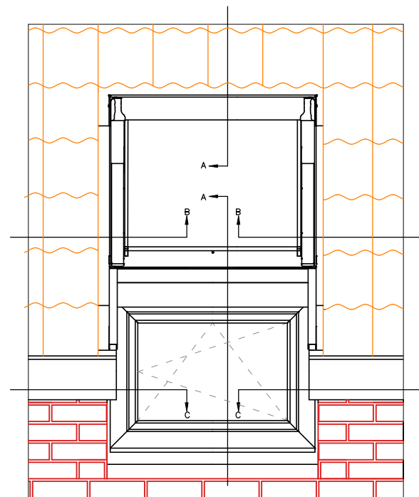
INDICATIVE SECTIONAL VIEW
