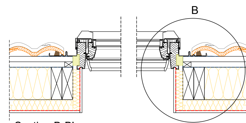
Section B-B' 1:10
