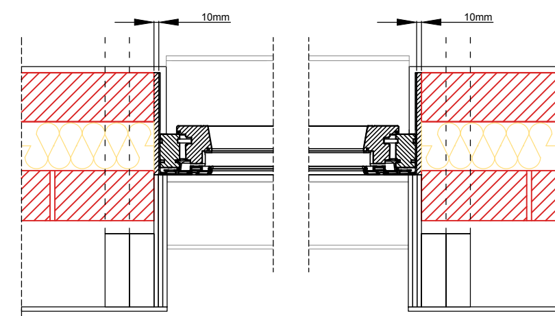
Section C-C' 1:10
