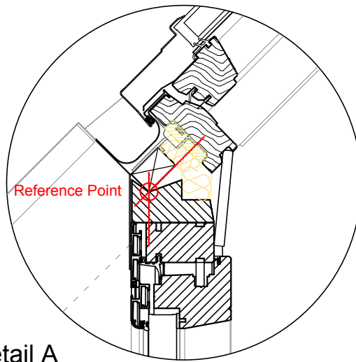
Detail A 1:5
