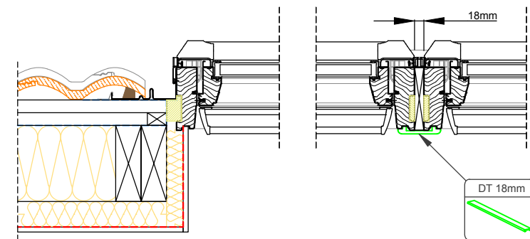
Section B-B' 1:10
