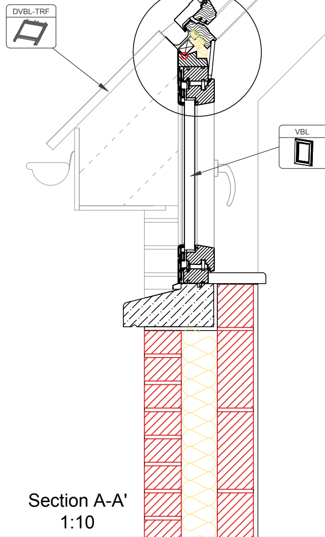
Detail B 1:5
