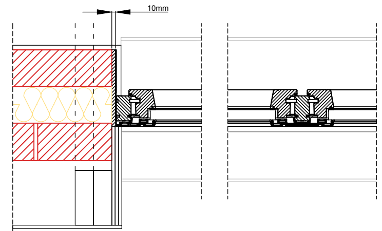
Section C-C' 1:10
