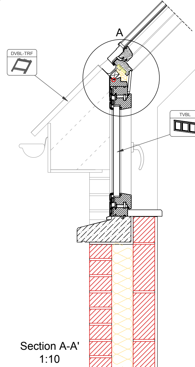
Detail A 1:5
