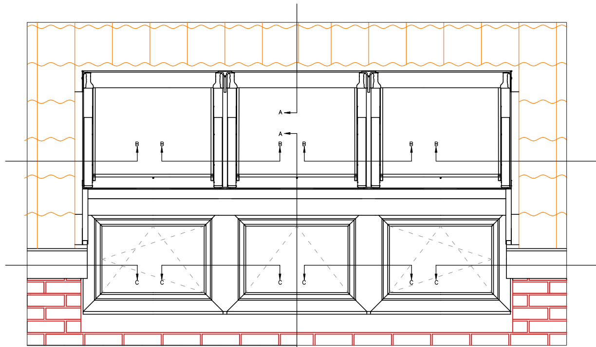
INDICATIVE SECTIONAL VIEW
