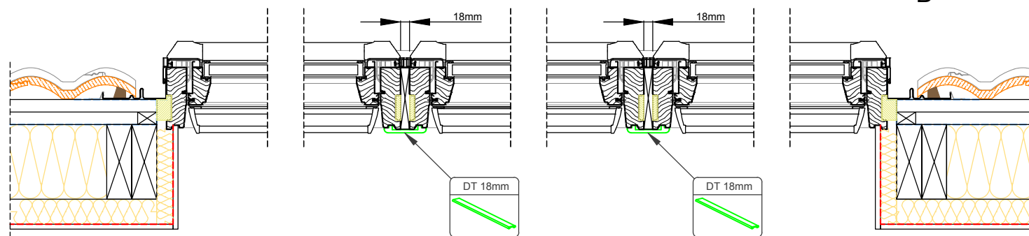
Section B-B' 1:10
