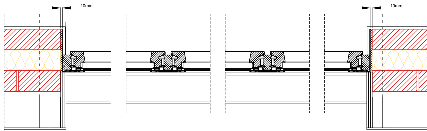
Section C-C' 1:10
