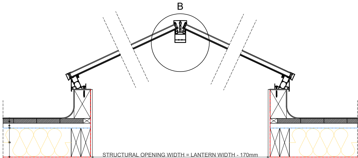
Section B-B' 1:10
