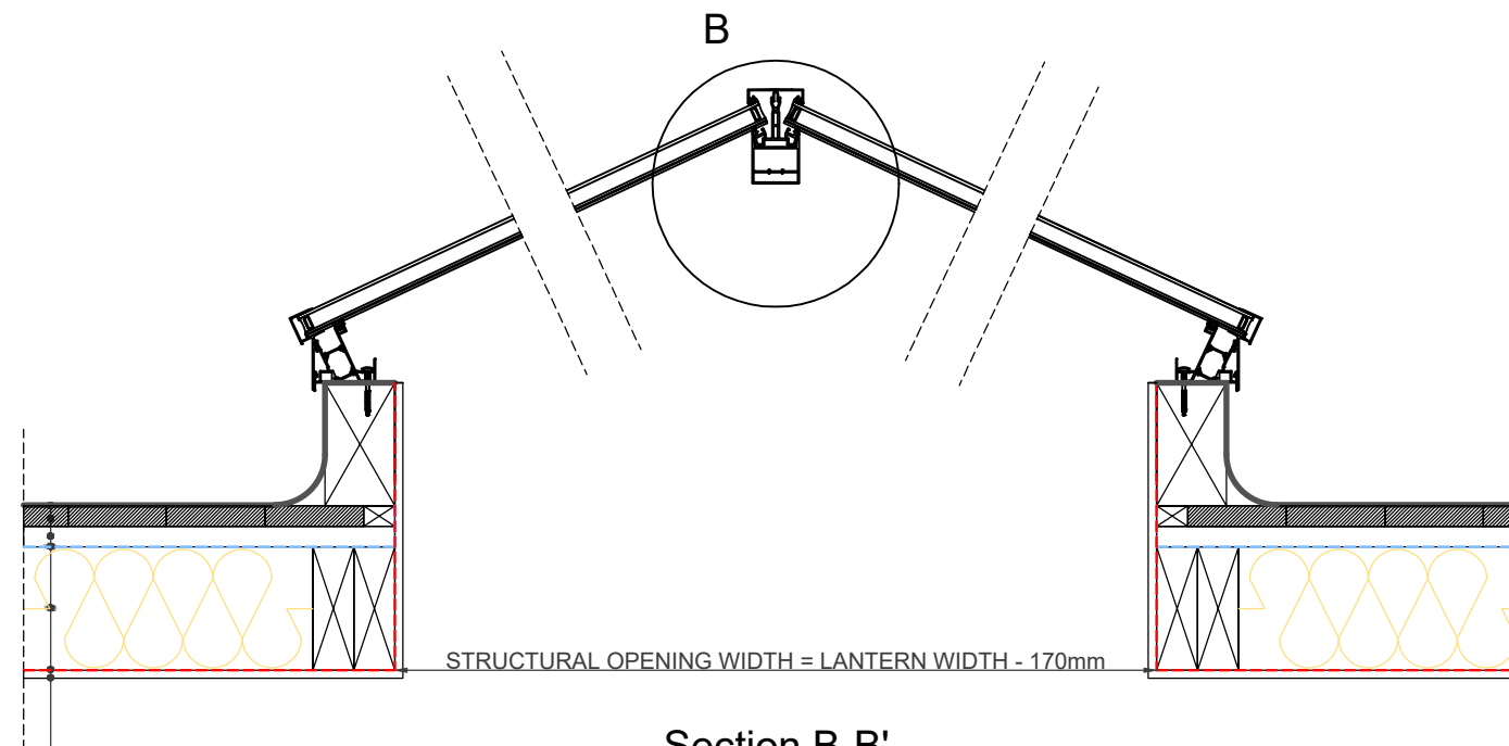
Section B-B' 1:10
