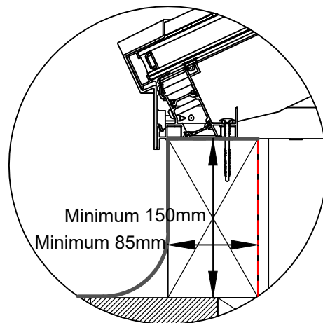
Detail B 1:5
