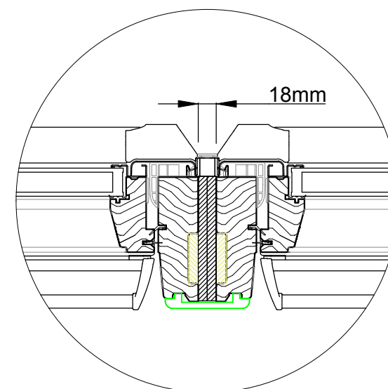
Detail A 1:5
