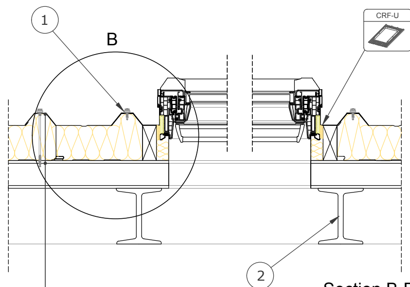
Section B-B' 1:10
