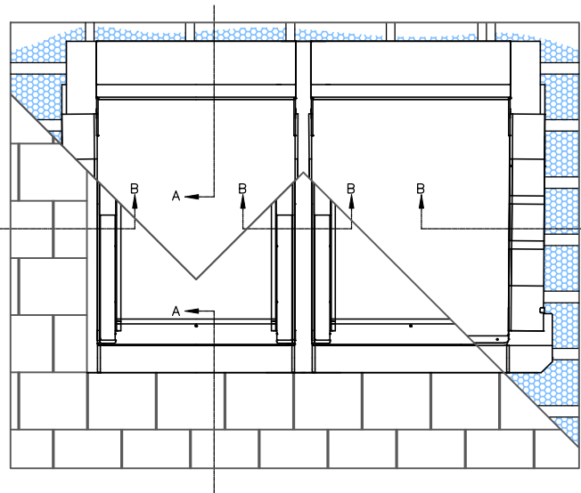
INDICATIVE SECTIONAL VIEW
