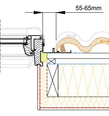
Section B-B' 1:10
