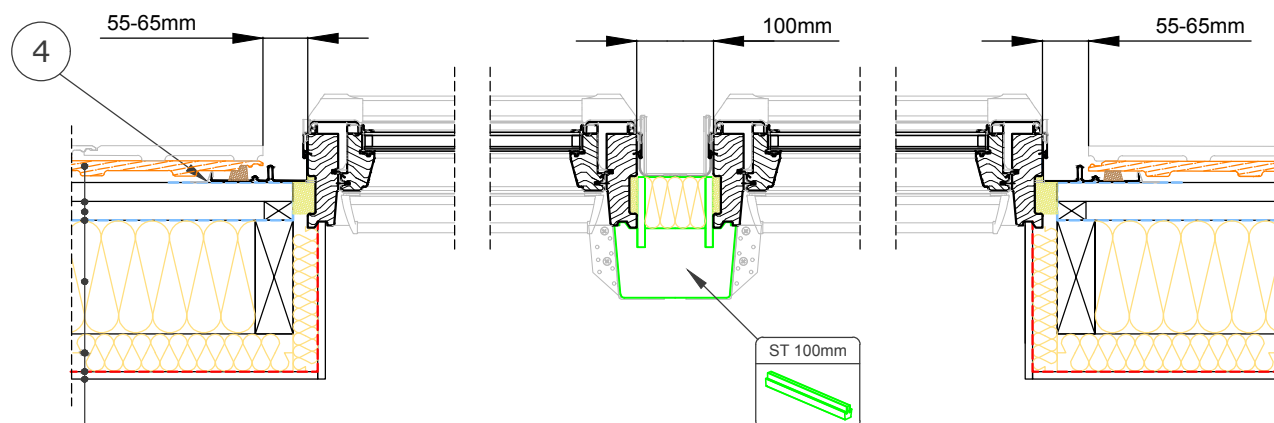
Section B-B' 1:10
