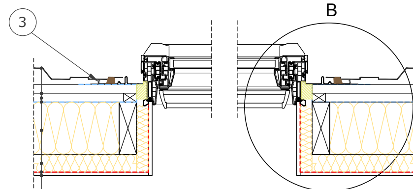
Section B-B' 1:10
