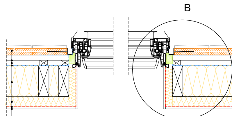
Section B-B' 1:10
