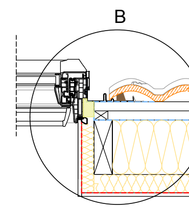
Section B-B' 1:10
