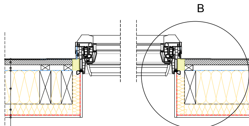
Section B-B' 1:10
