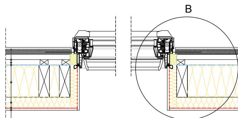
Section B-B' 1:10
