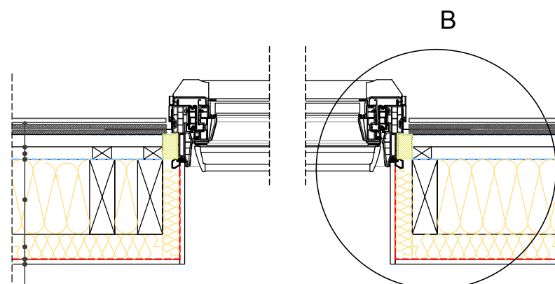
Section B-B' 1:10
