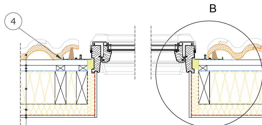
Section B-B' 1:10
