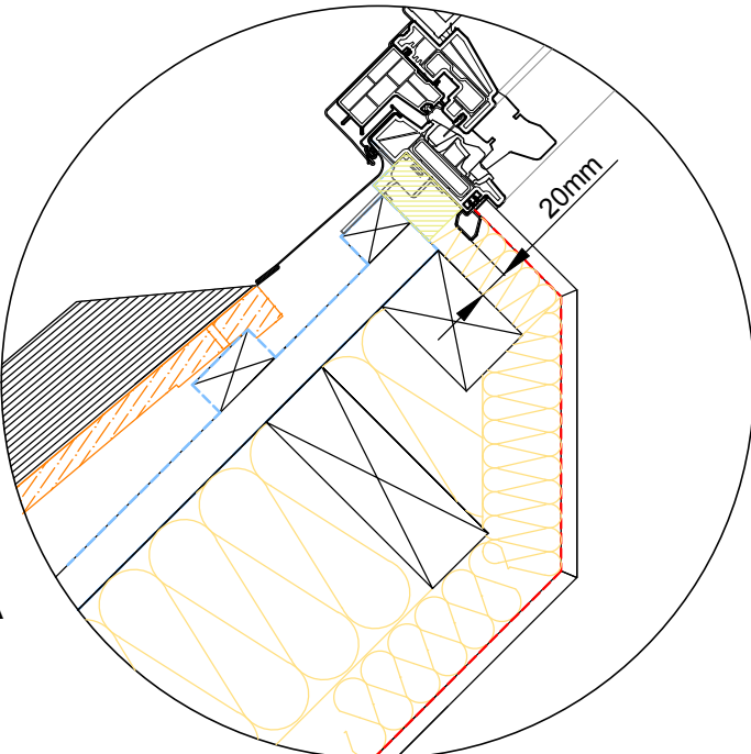
Detail A 1:5
