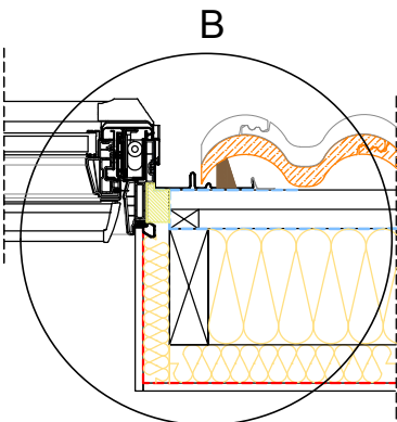
Section B-B' 1:10
