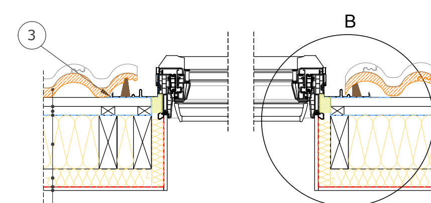
Section B-B' 1:10
