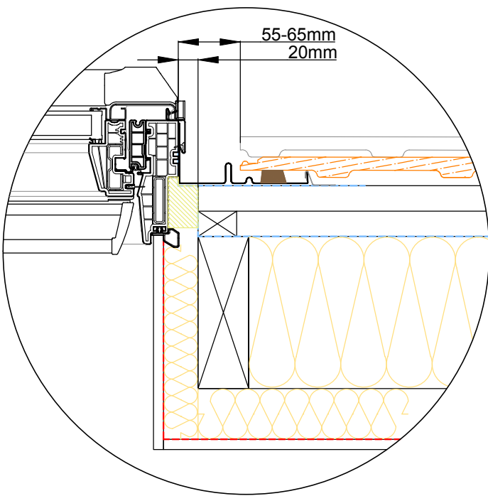
Detail B 1:5
