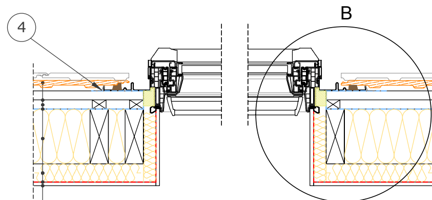
Section B-B' 1:10
