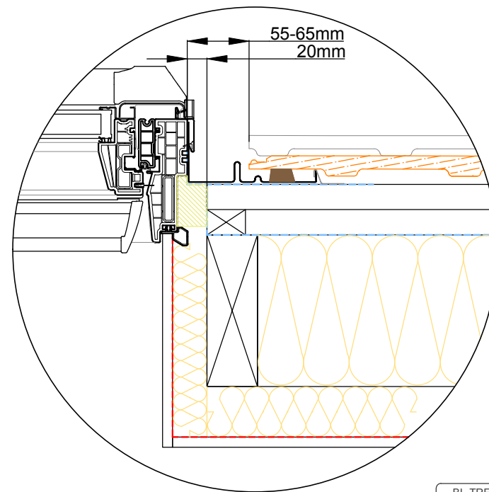
Detail B 1:5
