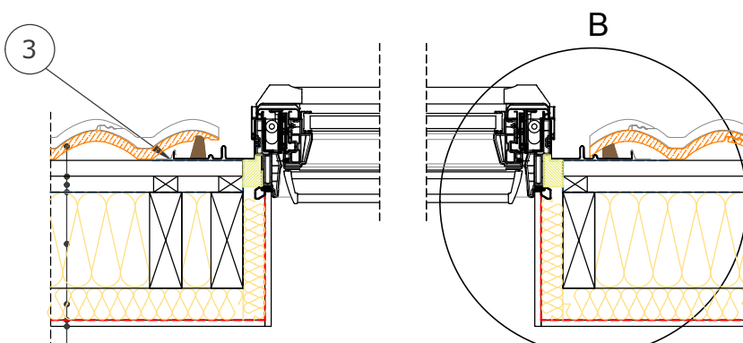
Section B-B' 1:10
