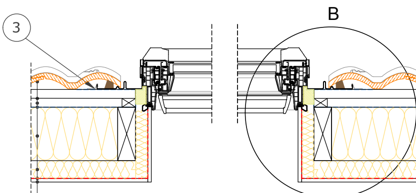
Section B-B' 1:10
