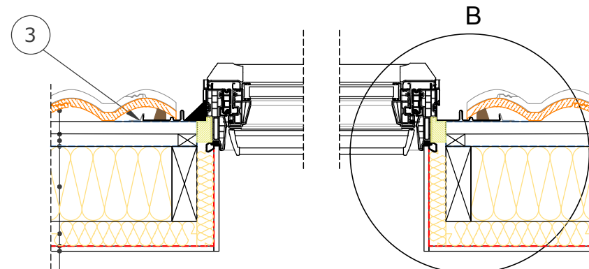
Section B-B' 1:10
