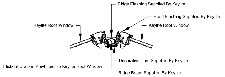
FRX RIDGE DETAIL
