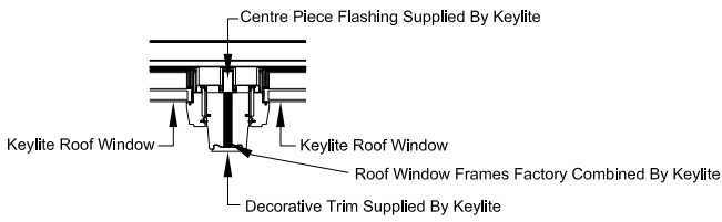
FRX ROOF WINDOW JOINT DETAIL
